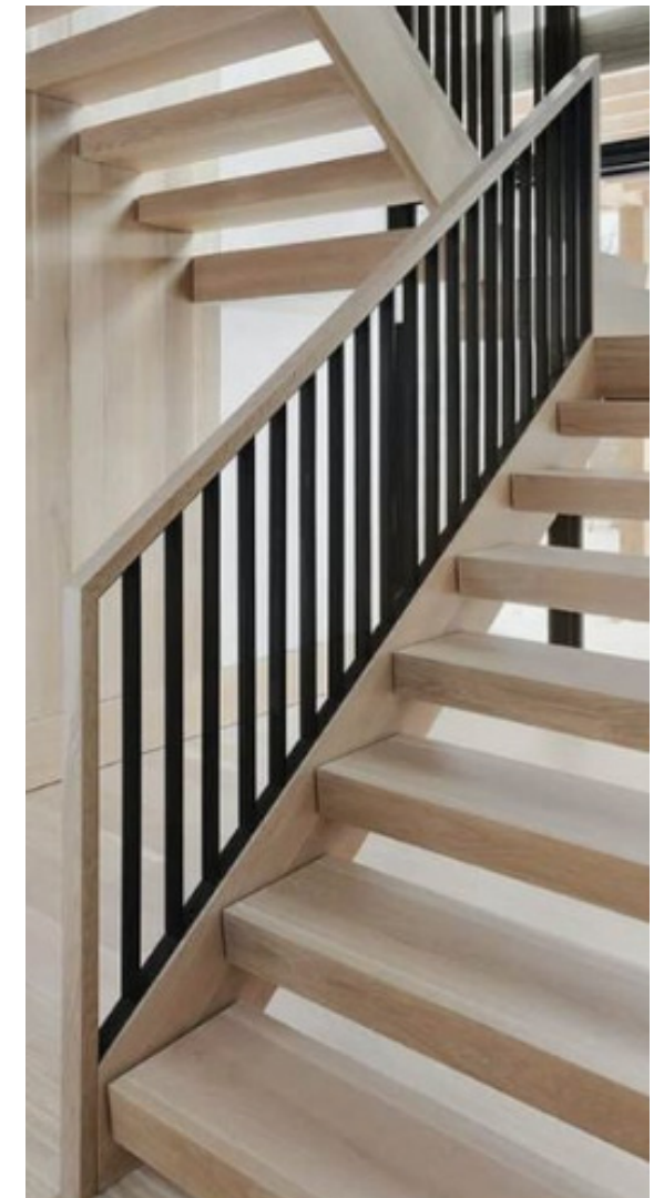
IRON RAILING 1"x 3/8" Thick Flat Iron Balusters, Iron plate at bottom of Balusters, Rift White Oak handrail, Stringer Open Textured Oak Wrapped Stair Treads
